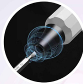
Strong magnetism
